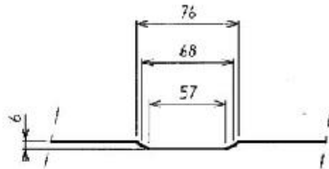
PILETTA 1"1/2
